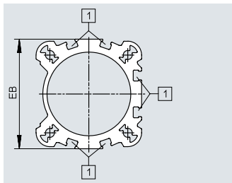
[1] Sensor slot for proximity switch
